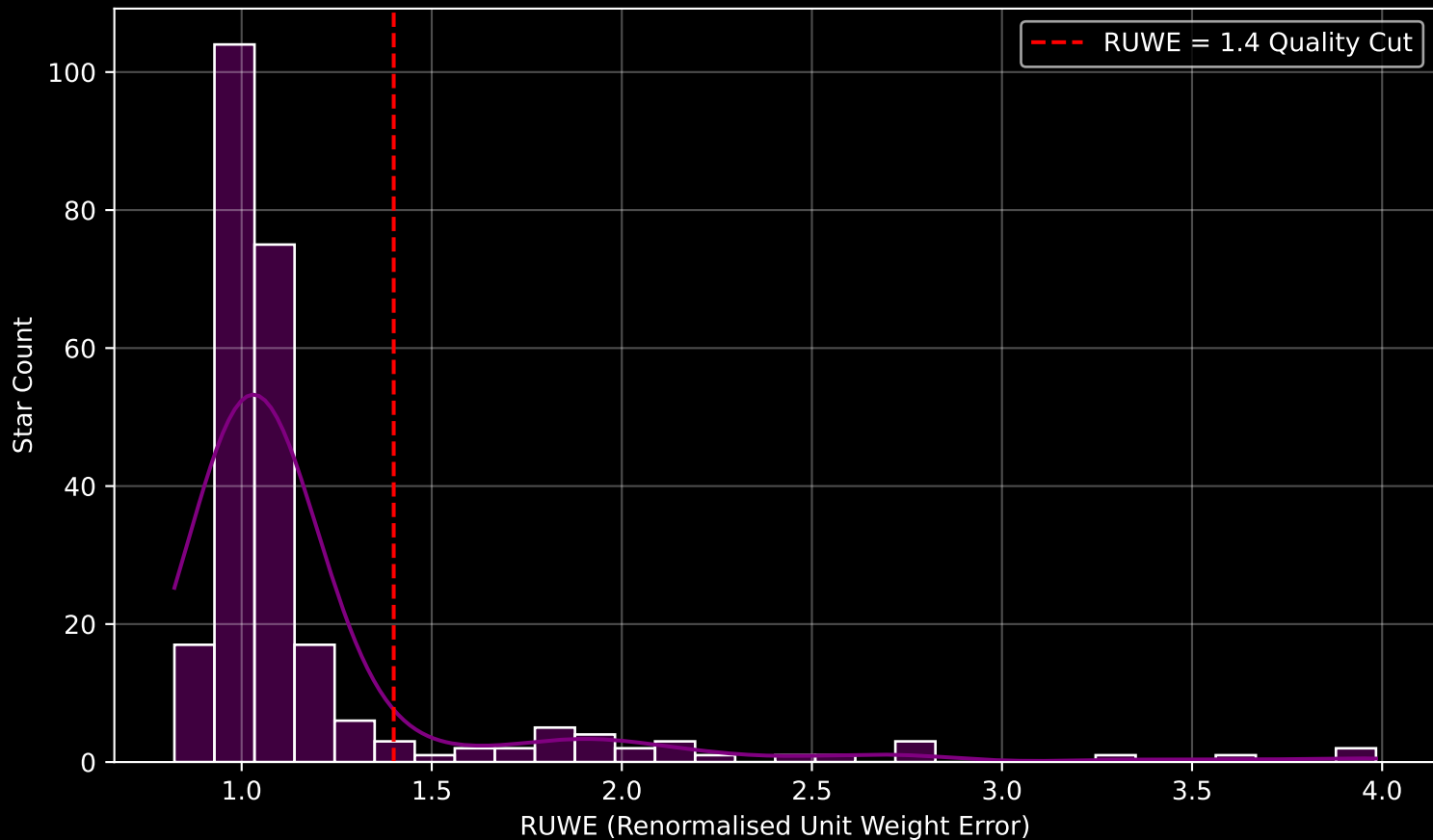
GALAH DR4 Field [2154] RUWE Distribution (n= 251)
