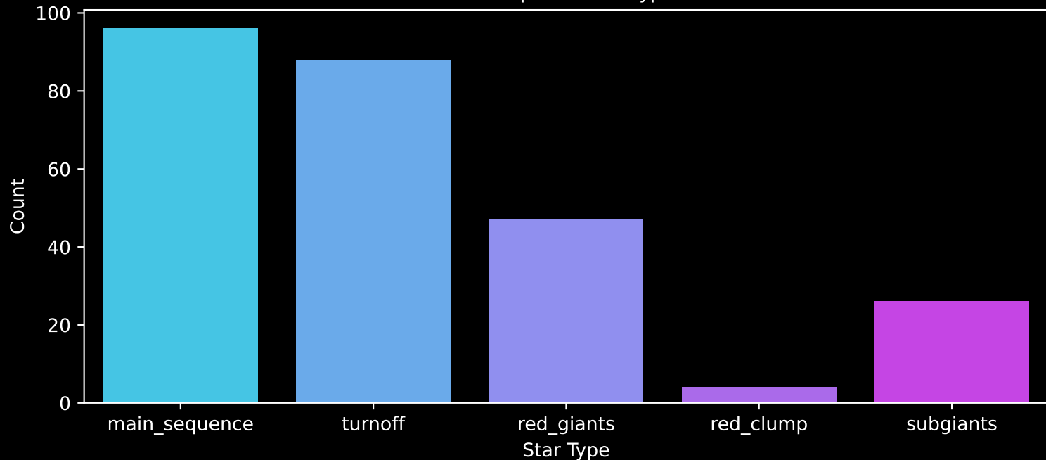
GALAH DR4 Field: [2154] Count plot of Star Type
